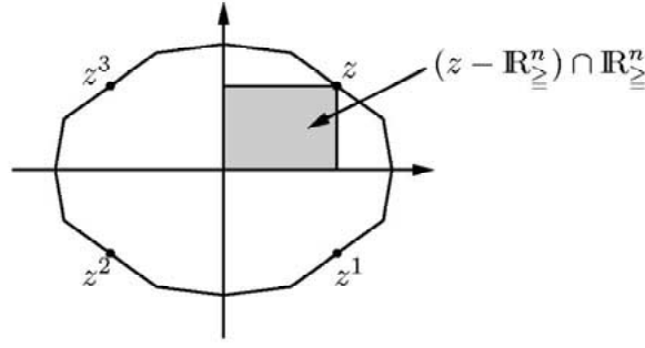
Figure 1. Example of the unit ball of an oblique norm \leftarrow with R(z) = \{z, z^1, z^2, z^3\} .
